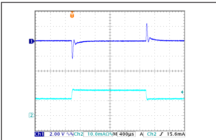
Figure 5: Output voltage response to step-change in load current (66% -100% -66% of I_{out(max)} ; dI/dt = 0.1 A/\mu s ). Load cap: 1 \mu F ceramic capacitor. Ch 1: V_{out} , Ch 2: I_{out} (2 A/div).
