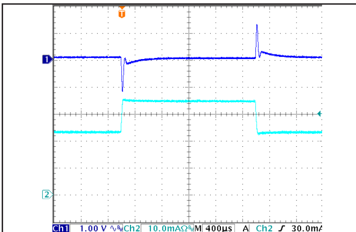
Figure 5: Output voltage response to step-change in load current (66% -100% -66% of Iout(max); dI/dt = 0.1 A/µs). Load cap: 1 µF ceramic capacitor. Ch 1: Vout, Ch 2: Iout (2 A/div).
