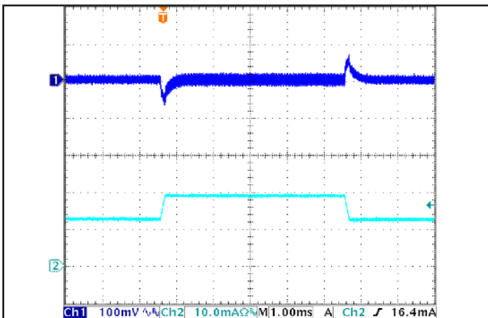
Figure 5: Output voltage response to step-change in load current (66% -100% -66% of I out (max); dI/dt = 0.1 A/μs). Load cap: 15 μF tantalum and 1 μF ceramic capacitors. Ch 1: V out , Ch 2: I out (20 A/div).
