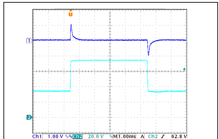
Figure 6: Output voltage response to step-change in input voltage (nominal to maximum, 1000 V/ms). Load cap: 1 µF ceramic capacitor. Ch 1: Vout, Ch 2: Vin.
