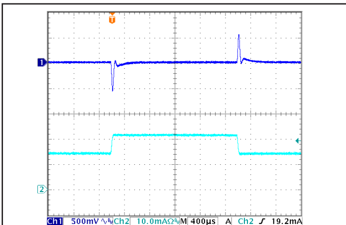
Figure 5: Output voltage response to step-change in load current (66% -100% -66% of I out (max); dI/dt = 0.1 A/μs). Load cap: 15 μF tantalum and 1 uF ceramic capacitors. Ch 1: V out , Ch 2: I out (5 A/div).
