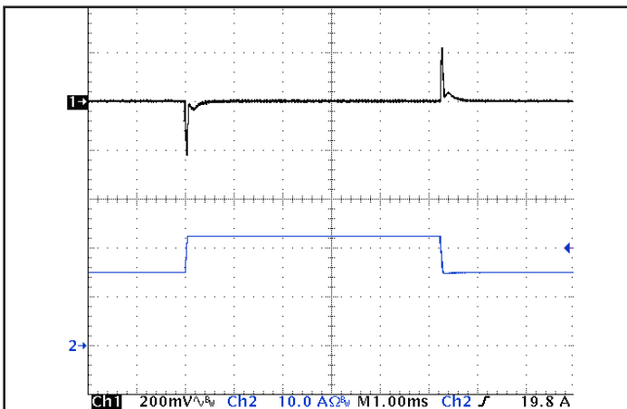
Figure 5: Output voltage response to step-change in load current (66% -100% -66% of I out (max); dI/dt = 0.1 A/μs). Load cap: 15 μF tantalum and 1 μF ceramic capacitors. Ch 1: V out , Ch 2: I out (10 A/div).
