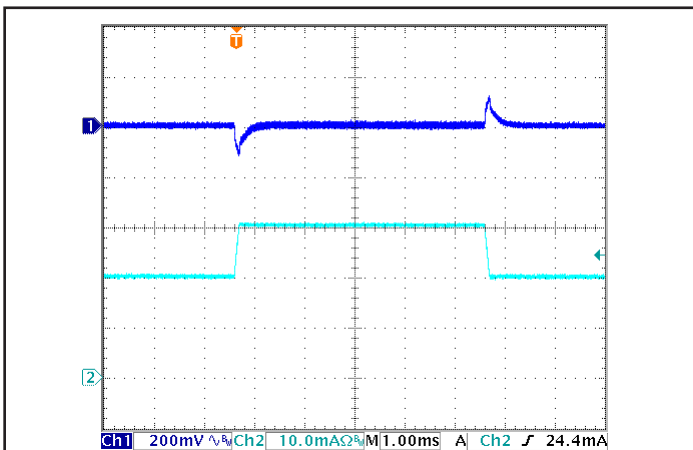
Figure 5: Output voltage response to step-change in load current (66% -100% -66% of Iout(max); dI/dt = 0.1 A/μs). Load cap: 15 μF tantalum and 1 μF ceramic capacitors. Ch 1: Vout, Ch 2: Iout (10 A/div).
