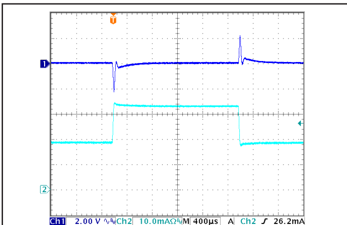
Figure 5: Output voltage response to step-change in load current (66% -100% -66% of I out (max); dI/dt = 0.1 A/μs). Load cap: 1 μF ceramic capacitor. Ch 1: V out , Ch 2: I out (1.5 A/div).
